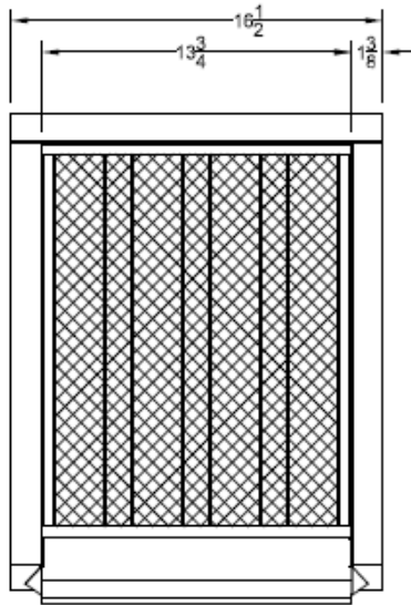
BACK VIEW
